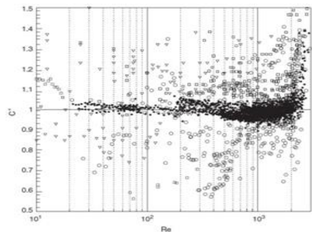
Fig 1. Symbols indicate geometry of channel: (○) circular microtubes, Sharp & Adrian,2004; (o) circular microtubes, Judy et al.,2002; (Δ) trapezoidal microchannels, Qu et al.,2000; (□) rectangular microchannels, Liu & Garimella,2004. Above all, it can be concluded that the conventional theory for macroscale phenomena can be applied to smooth-walled microchannels. However, there is a need for more
