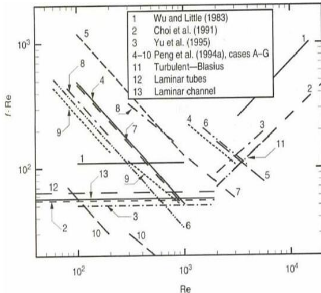
Fig 2. Comparison of the fluid friction characteristics from various investigations on convective flow in microchannels (From Sobhan, C.B. and Garimella, S.V., Microscale Thermophys. Eng. , 5, 293, 2001.)
