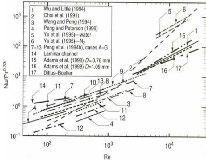
Fig 3. Comparison of the heat transfer characteristics from various investigations on convective flow in microchannels. (From Sobhan, C.B. and Garimella, S.V., Microscale Thermophys. Eng. , 5,293, 2001.)
